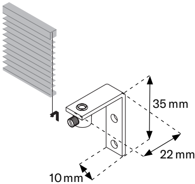
Side guiding fitting | Wall Metal colour or white
