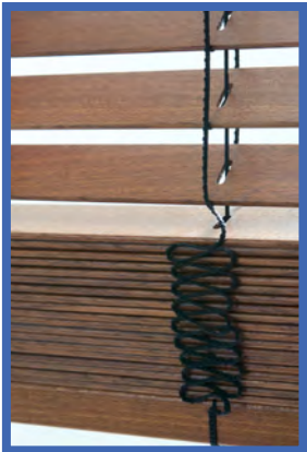
25 mm slat width with thin ladder cord
